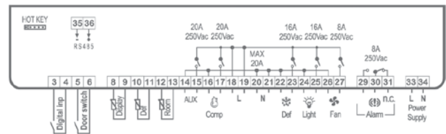
direct load
