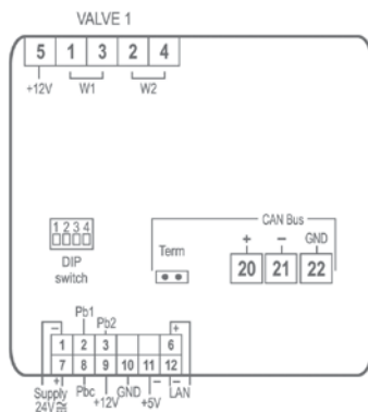
XEV20D - 1 circuit
